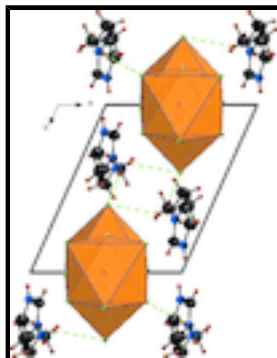
Fig. 2. The crystal packing of (C_6H_{13}N_3)_2Pb_3I_{10} viewed along [001] direction and showing the N—H...I hydrogen bonding (dashed lines).
